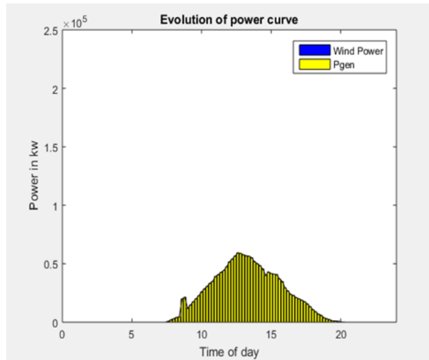
Figure 5 Time of Day vs Power in kW.
