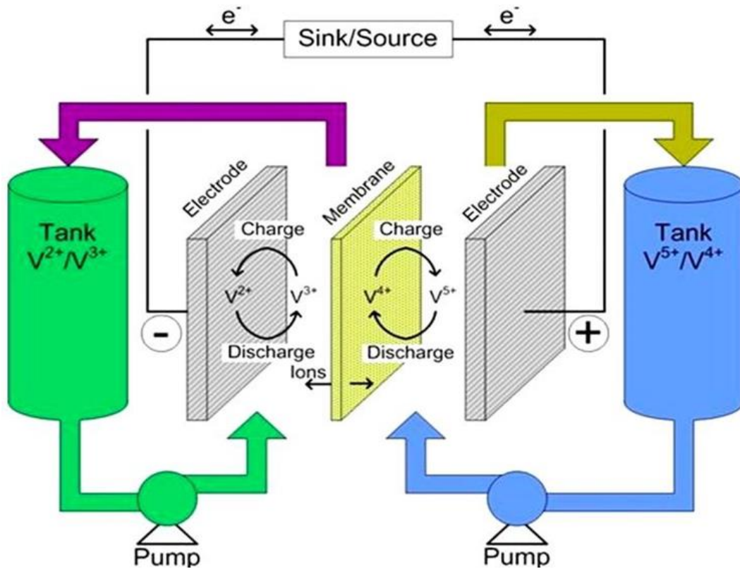
Figure 2 Vanadium Redox Battery.
