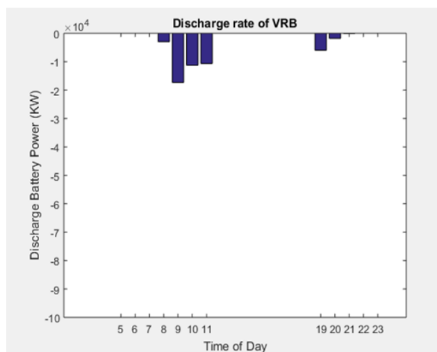
Figure 7 Model of VRB Battery.
