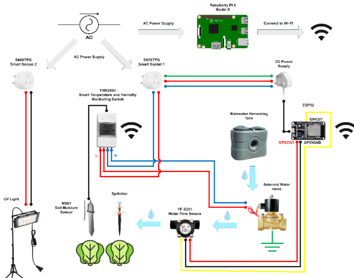
Figure 1 Proposed architecture connection and operation of outdoor home smart farming based on Raspberry Pi for Home Assistant management.
