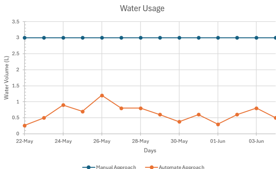
Figure 4 Daily water usage for both manual and automated approach to cultivate the Pak Choi vegetables.
