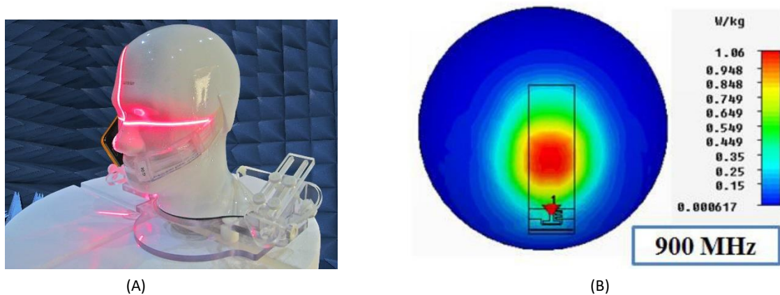
Figure 1 SAR assessment methods (A) Physical measurements, http://www.indexsar.com (B) Simulation measurements.
