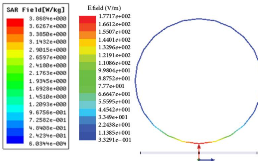
Figure 17 Measurement of the E-field in the fat layer of the child's head.
