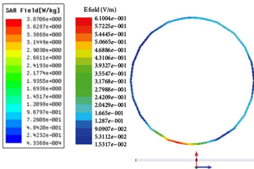
Figure 14 Measurement of the E-field in the CSF layer of the adult head.
