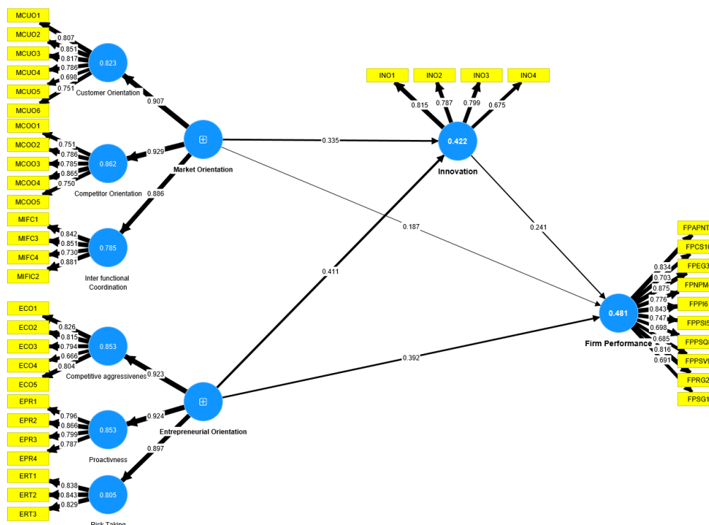
Figure 2 Measurement Model.
