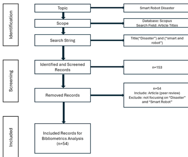
Figure 1 PRISMA diagram used in this review.
