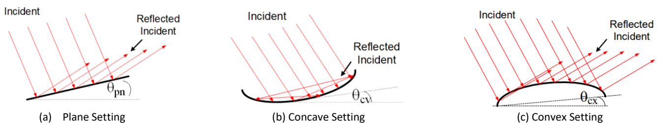
Figure 10 Incidents recorded by a solar panel with various surface configurations.
